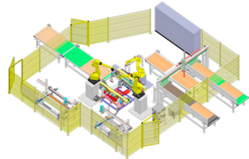
Tending system for clamping machine for 5 elements cabinet doors
